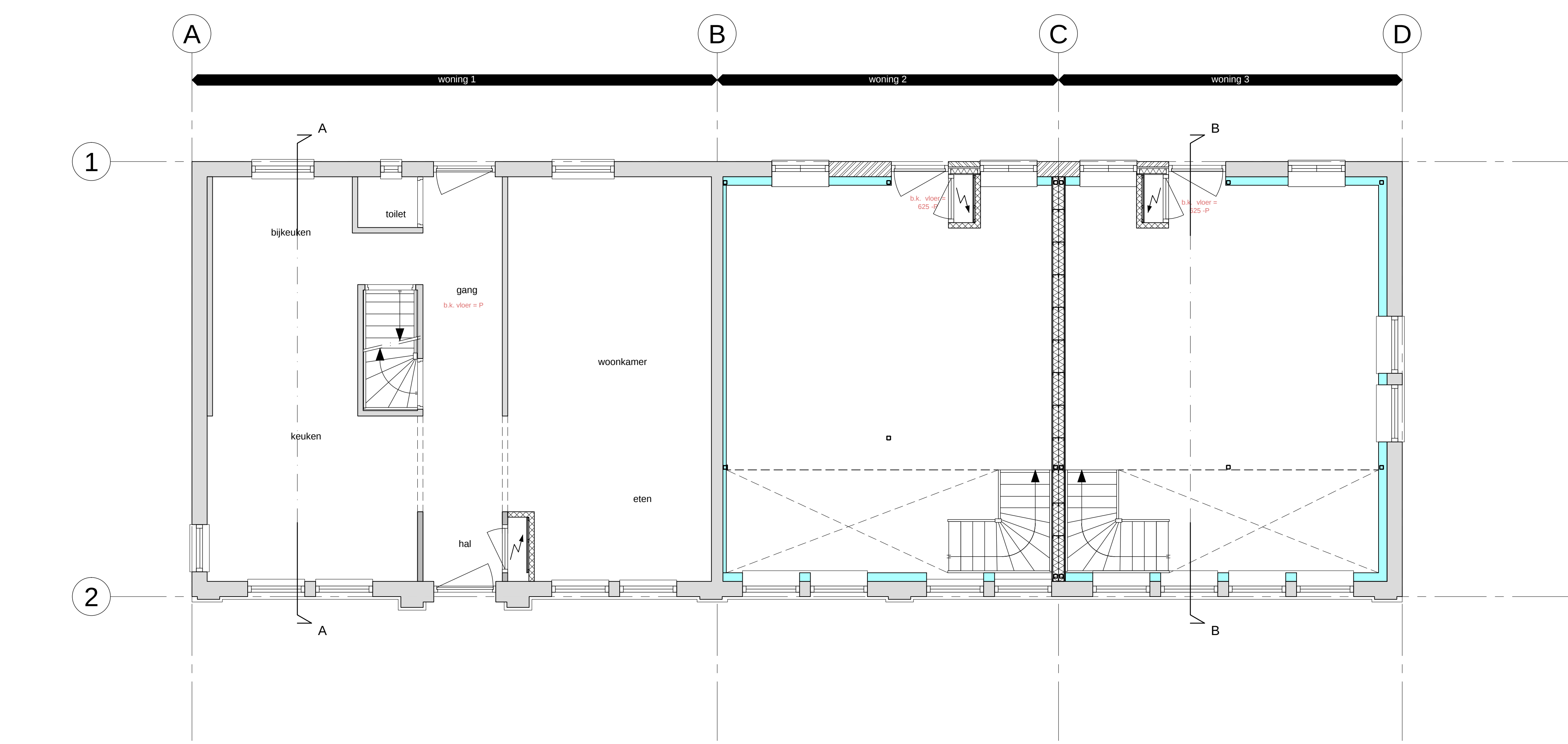
begane grond (1:50)
